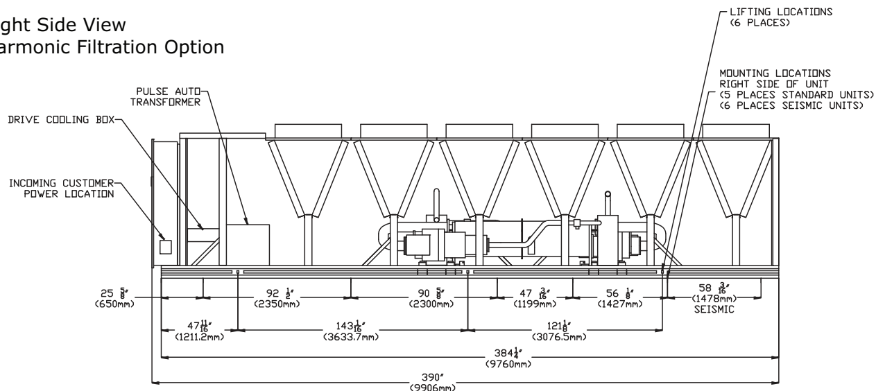
Figure 9. 200 to 250 ton — extended length unit
