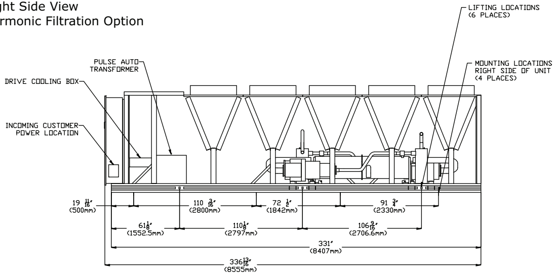
Figure 8. 165 and 180 ton — extended length unit
