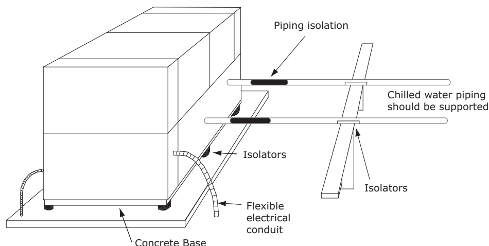
Figure 4. Installation example
