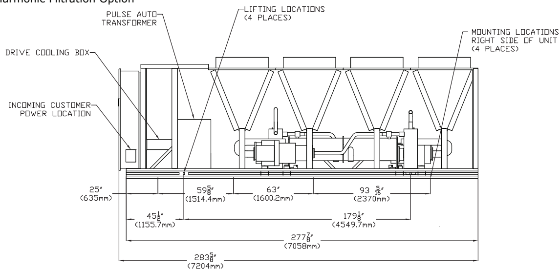
Figure 7. 150 ton — extended length unit
