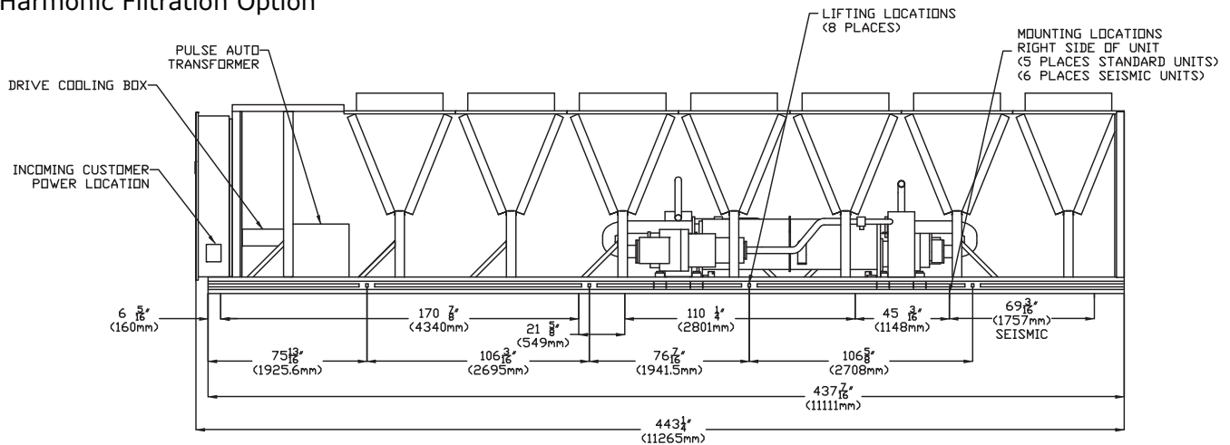
Figure 10. 275 ton — extended length unit
