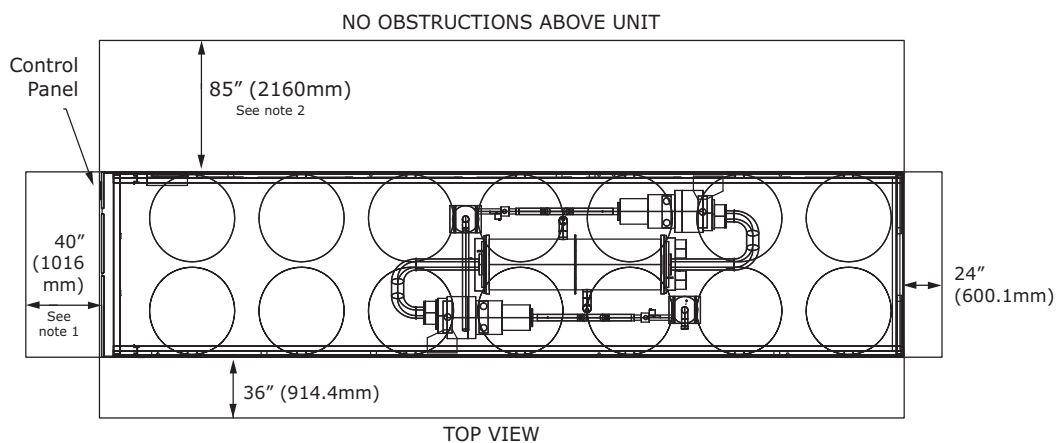
Figure 1. RTAE service clearances
